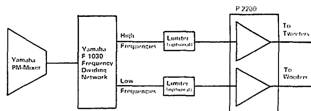
Fig. 66 - Biamplified System showing Placement of Optional Limiters.
