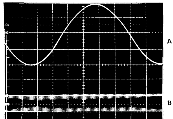
Fig. 64A - System using Conventional, Passive/High-Level Frequency Dividing Networks.
