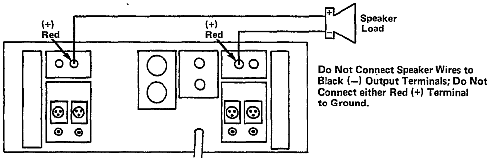
Fig. 63B - Output Connections for Operating P-2200 in "Mono" Mode.
