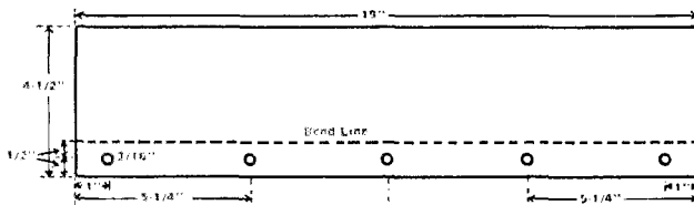
Rear fan air containment panel front view, before folding.
