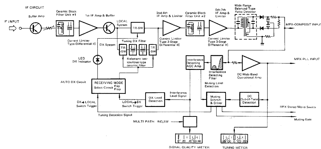
Block Diagram of AUTO DX Circuit
